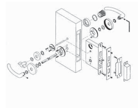
Figure 26 ML F RPS trim
