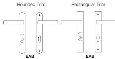
EAB Entry Set-Key below Entry function with American cylinder below the lever, 92mm center to center.
