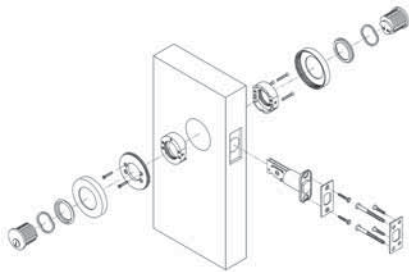
Figure 6 Double Cylinder 102 RP trim
