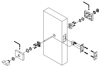
Figure 23 Privacy Bolt 105 RSQS
