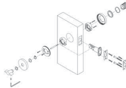
Figure 24 Deadbolt Single Cylinder 101 RPS
