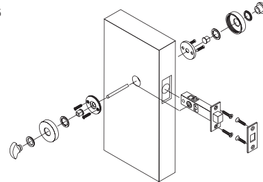
Figure 7 Privacy Bolt 105 RSP trim
