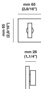
101 RQ / K1225 Solid brass
