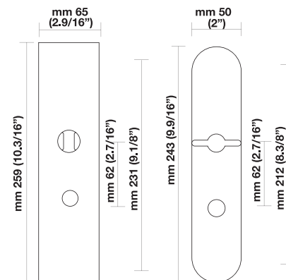
Stainless steel NES Narrow Plain Escutcheon
