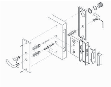
Figure 25 ML F ERS trim
