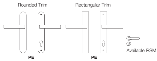
PE Patio Set-Profile cylinder no key Patio function with 1/2 profile cylinder and thumbturn, no keyway on the exterior plate.
