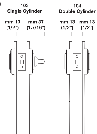
ERS - 103 Rectangular Escutcheon Stainless steel (shown w/H 5004 Door lever)
